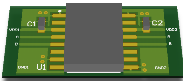
Figure 5.3 Recommended PCB Layout — Top Layer
